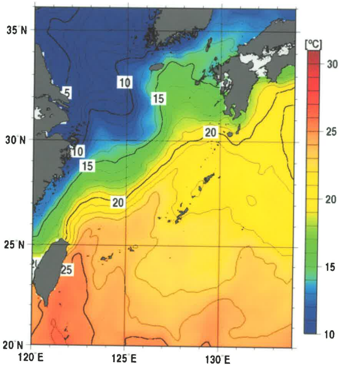
Monthly Mean SSTs for Feb. 2013.
