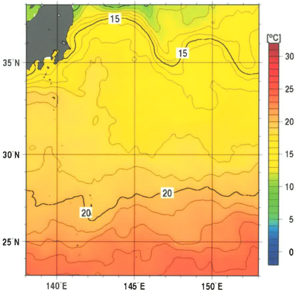
Monthly Mean SSTs for Feb. 2013.
